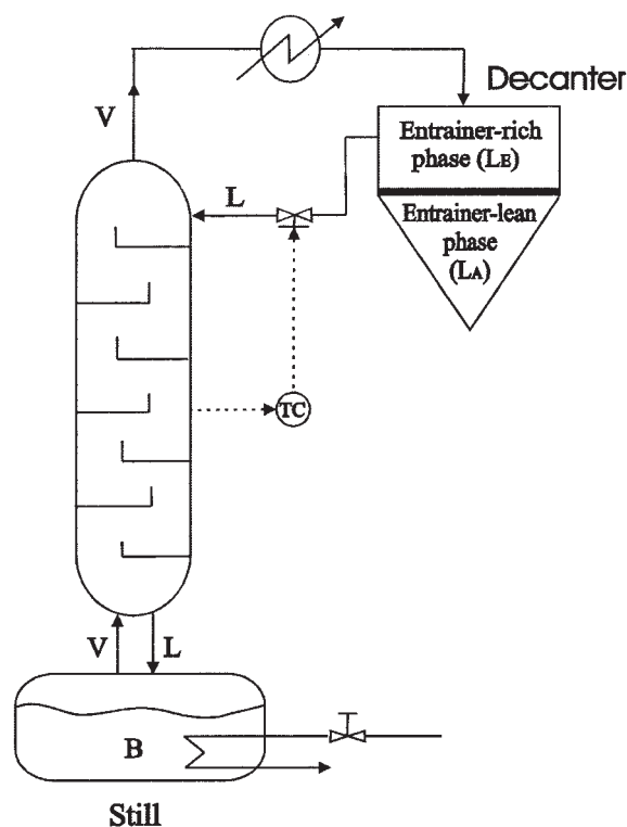
Figure 1. Batch rectifier column with the proposed control scheme.
