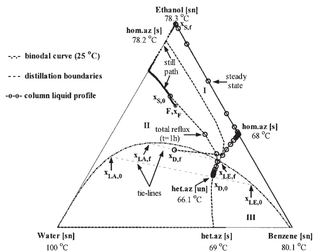
Figure 8. Separation of ethanol/benzene/water in the rectifier column.
